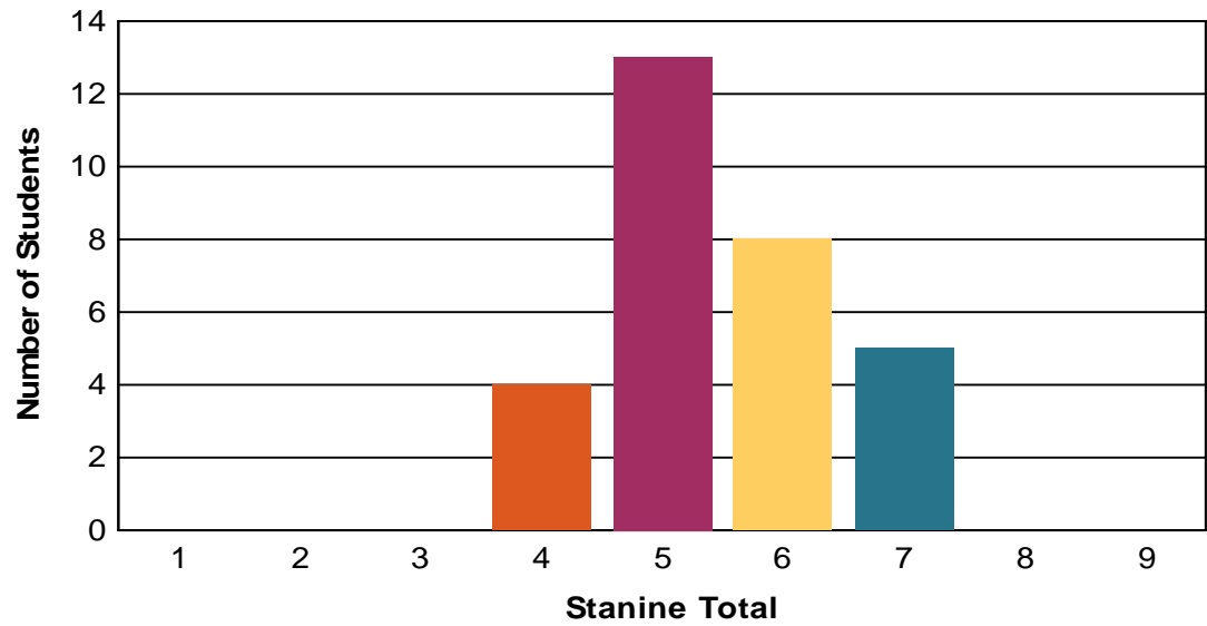
Stanine Distribution
